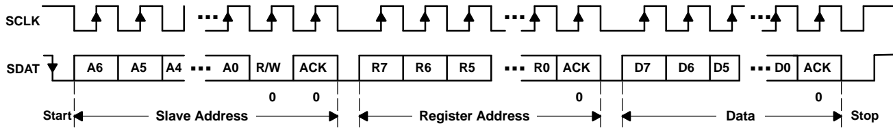
Figure 41. Serial Interface WRITE to TPS65011 Device
