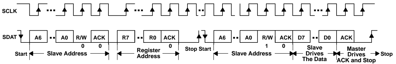
Figure 43. Serial Interface READ From TPS65011: Protocol B
