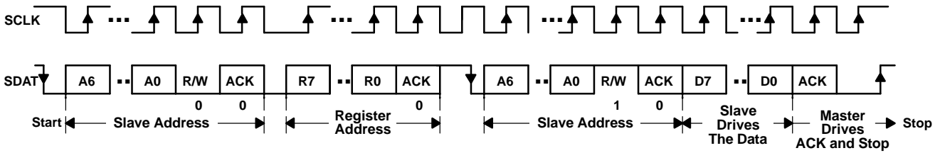
Figure 42. Serial Interface READ From TPS65011: Protocol A
